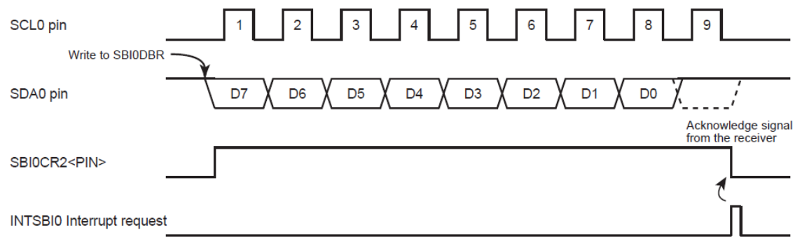
图 14- 18 SBI0CR1<BC>="000"与 SBI0CR1<ACK>="1" 传输
